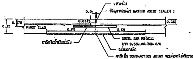
ขยายแสดง CONSTRUCTION JOINT AND CONTRACTION JOINT
